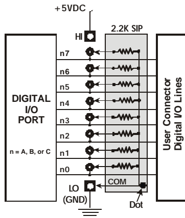
2.2K SIP INSTALLED FOR PULL-DOWN
