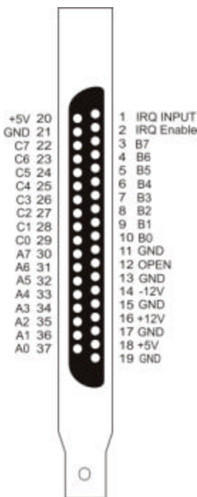
Figure 3-1. PCI-DIO24/PCI-DIO24H Series Connector Pinout
