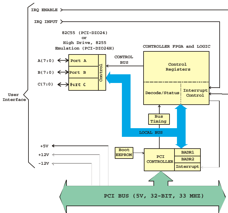
Figure 1-1 PCI-DIO24 and PCI-DIO24H Functional Block Diagram
