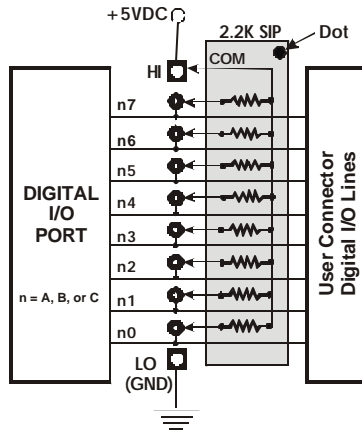
2.2K SIP INSTALLED FOR PULL-UP
