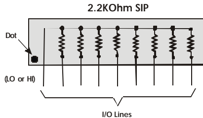
Figure 3-3. Eight-Resistor SIP Schematic
